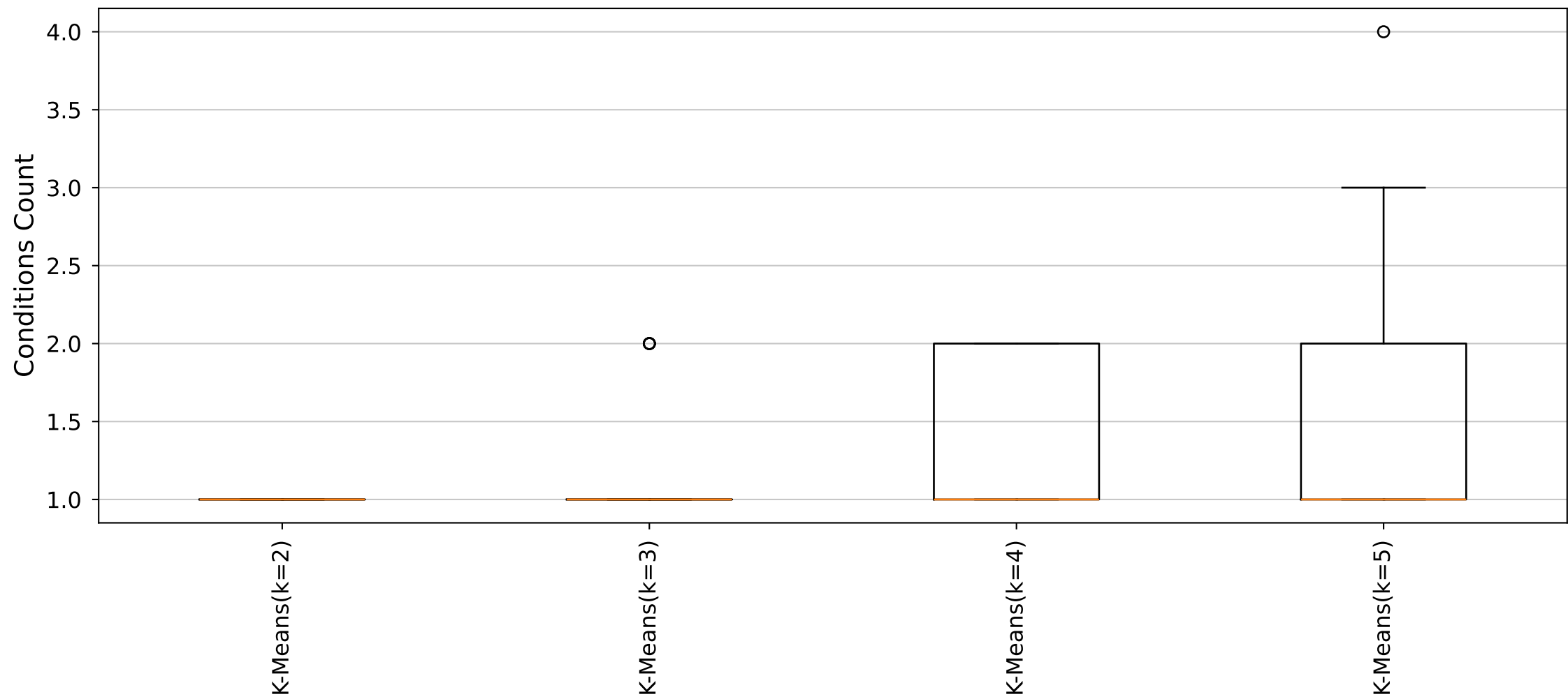
YARA Rules Conditions Count Distribution (Cluster41_Size5 dataset)
